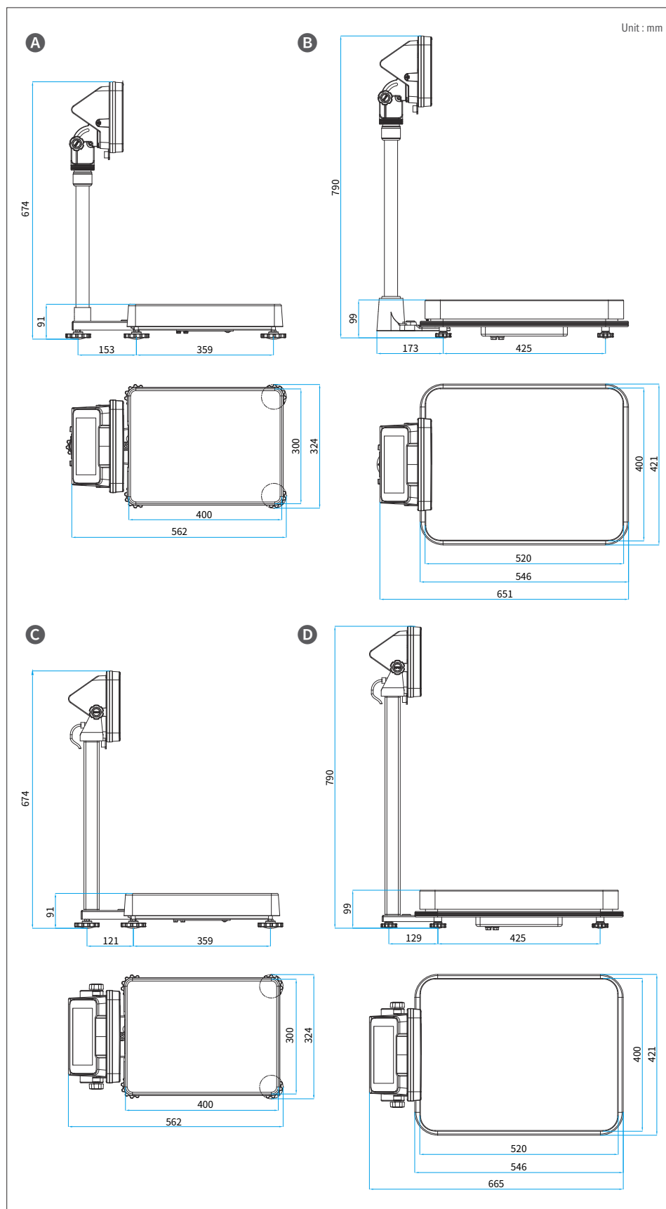
B EBW-60/150AD (Round shape post pipe)
